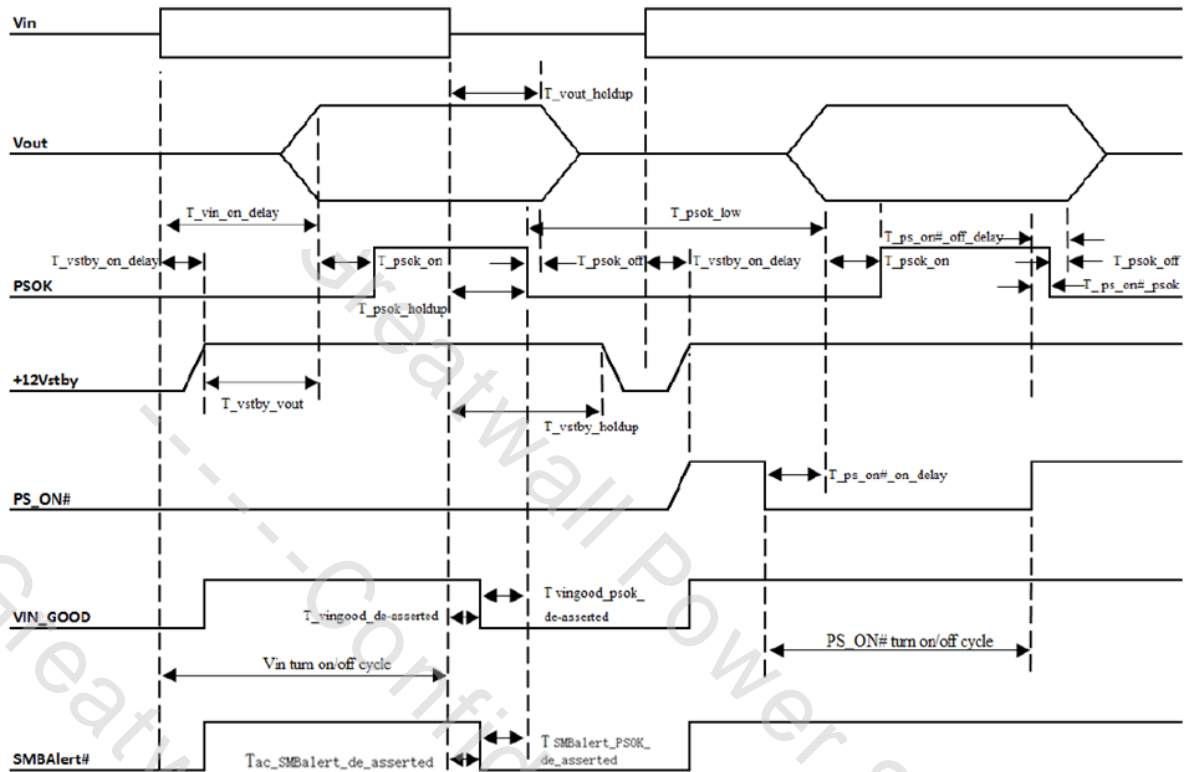
Figure 8 Turn On/Off Timing
