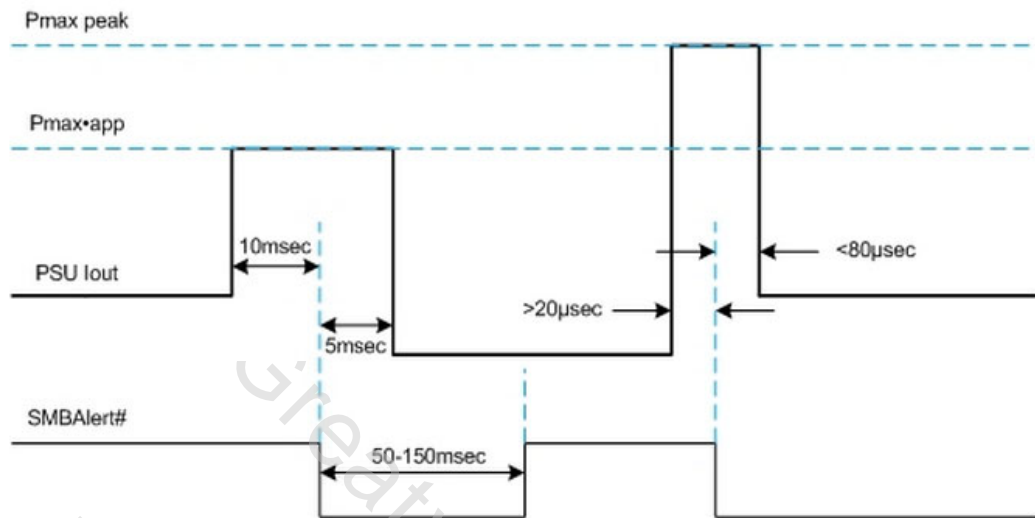
Figure 7 PSU Peak Timing
