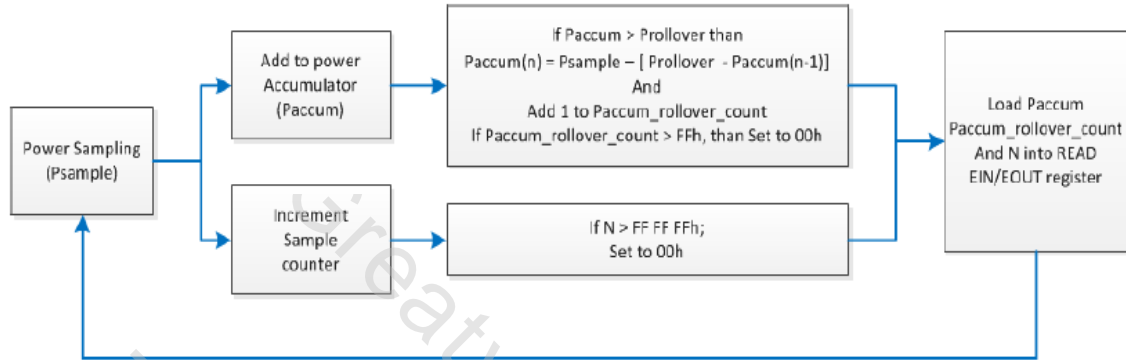
Figure 10 Read_EIN Functional Diagram
