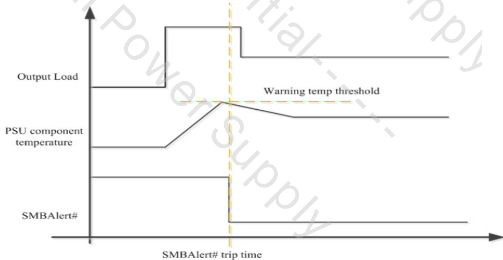
Figure 14 CLST Timing Requirement
